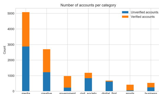
Figure 1: Category-Wise Counts
